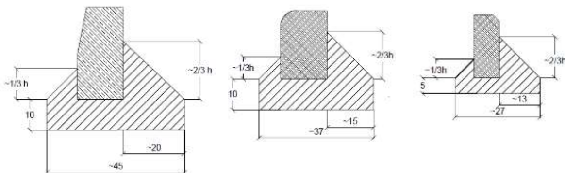
Betona apmale 100x30x15 cm
